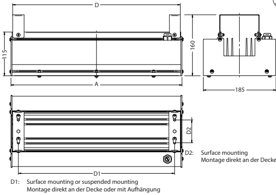
ATENA LINE LED 24000LM SH MEDIUM E IP65 750
